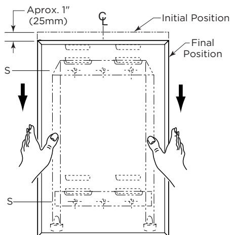
Snap Locking Design (Front View)
