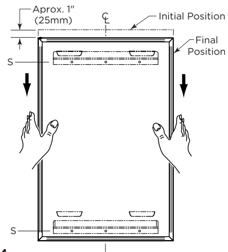
"2S"-Tab Design - up to 36" Width (Front View)
