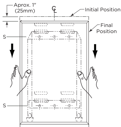
Snap Locking Design (Front View)
